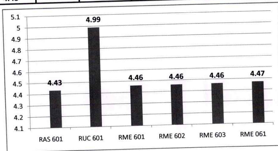
THEORY
